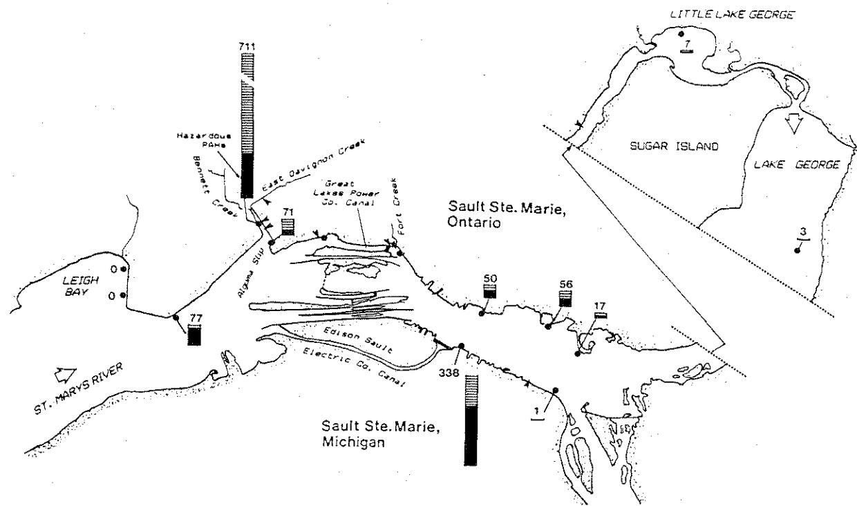
Fig. 3. Total polycyclic aromatic hydrocarbons ( \text{mg kg}^{-1} , dry wt) in surficial sediments of the St. Marys River in 1985. Bar height is proportional to concentration; shaded portion of bars indicates the proportion of the total comprised of mutagenic and/or carcinogenic compounds.
